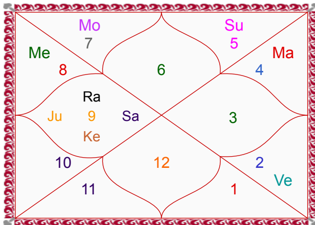
Panchamsa Chart
